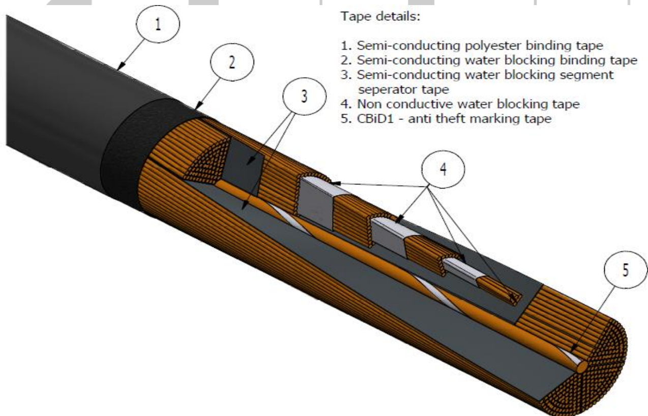
Figure 1: Typical construction of the water blocked Milliken conductor.
